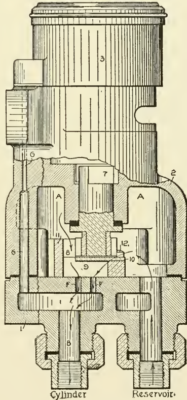
Fig. 94. Section of Air Operating Valve
